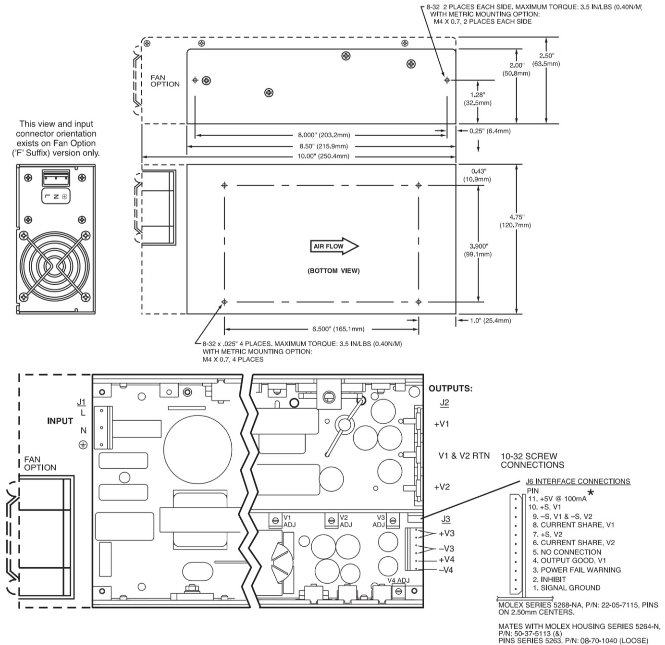
Figure 1 – Mechanical Drawing PFC250
