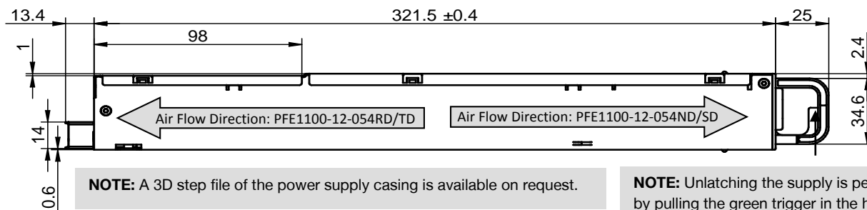
Figure 3 - Side View 1
