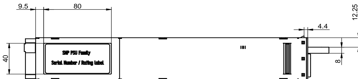
Figure 3 - Side View 1
