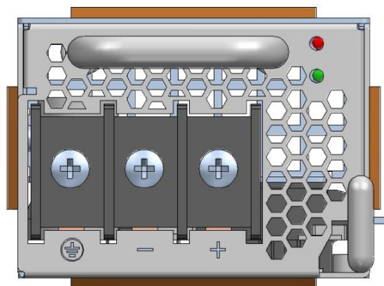
Figure 7 - Front View (PFE1100-12-054SD/TD)
