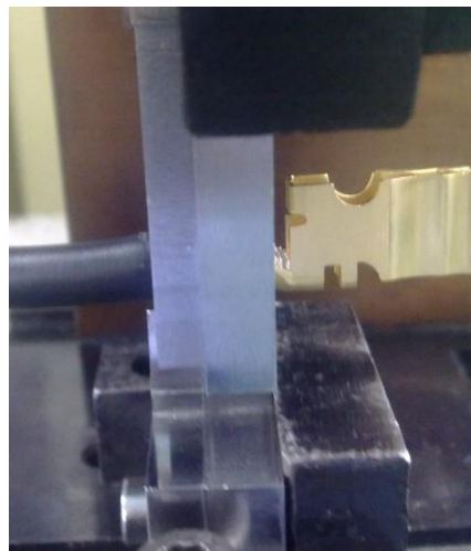
Picture 6 - Positon after crimped
