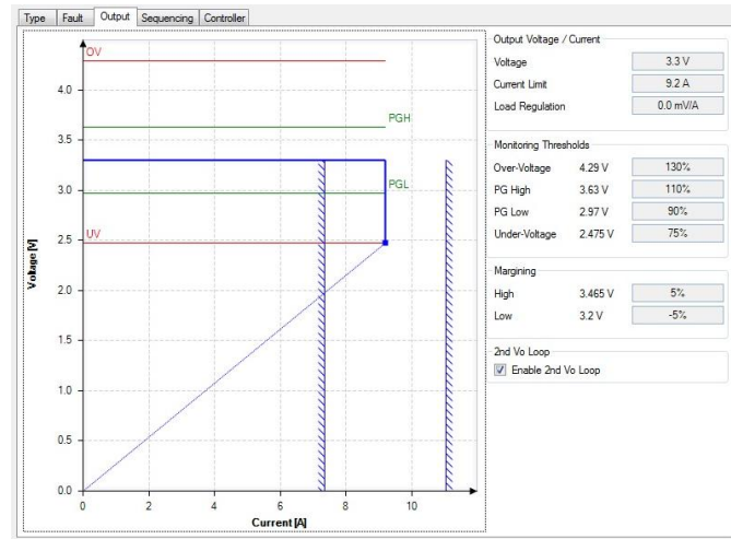
Figure 6. Output Configuration Window
