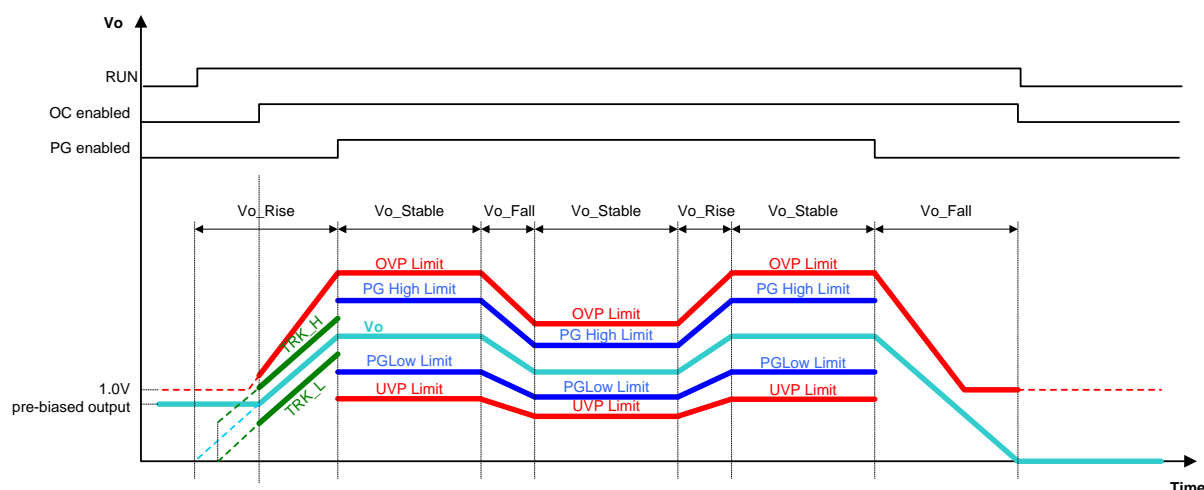
Figure 25. Protection Enable Conditions
