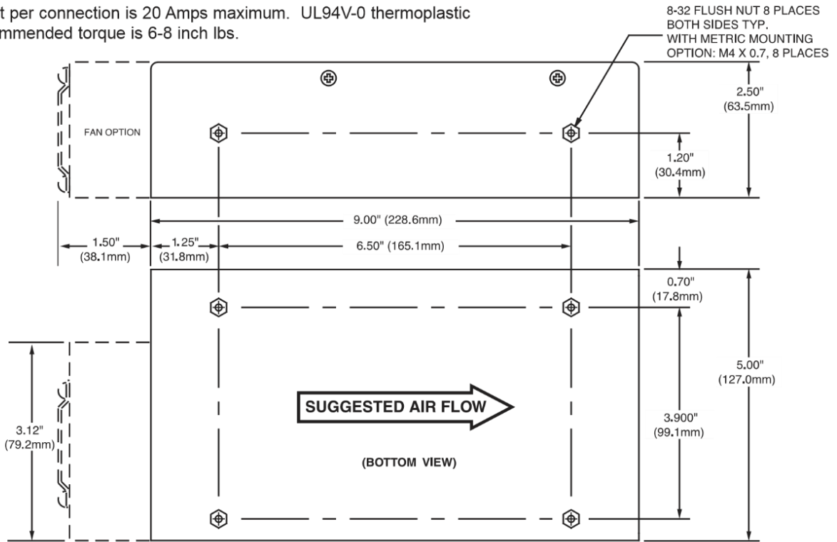
Figure 1 – Mechanical Drawing PFC375
