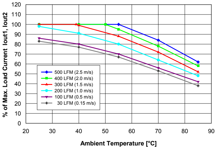
Fig. 14: Available balanced load current (Iout1 = 1.5·Iout2) vs. ambient air temperature and airflow rates for converter mounted vertically with Vin = 48 V, air flowing from pin 3 to pin 4 and maximum FET temperature ≤ 120°C.
