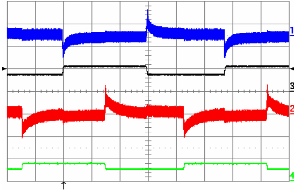
Fig. 28: Output voltage response to both Iout1 and Iout2 (out of phase) load current step-change of 3.75 A (Iout1) and 2.5 A (Iout2) (50%-75%-50%) at V_{in} = 48 V. Ch1 = Vout1 (50 mV/div), Ch2 = Vout2 (50 mV/div), Ch3 = Iout1 (10 A/div.), Ch4 = Iout2 (10 A/div.). Current slew rate: 0.1 A/ \mu s, C_o = 10 \mu F tantalum + 1 \mu F ceramic. Time scale: 1 ms/div.
