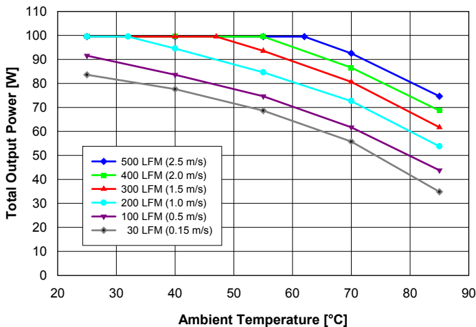
Fig. 1: Available output power vs. ambient air temperature and airflow rates for QD48T033050 converter mounted vertically with air flowing from pin 3 to pin 1, MOSFET temperature \leq 120^{\circ}\text{C} , V_{in} = 48\text{ V} and balanced load on both outputs ( I_{out1} = 1.5 \cdot I_{out2} ).
