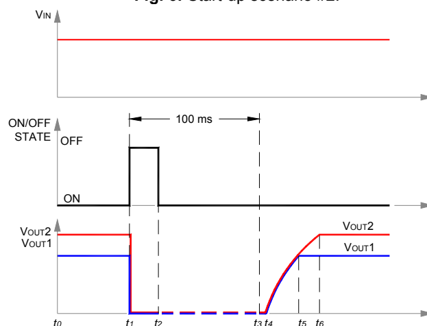
Fig. 7: Start-up scenario #3.
