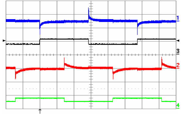
Fig. 29: Output voltage response to both Iout1 and Iout2 (out of phase) load current step-change of 3.75 A (Iout1) and 2.5 A (Iout2) (50%-75%-50%) at V_{in} = 48 V. Ch1 = Vout1 (100 mV/div), Ch2 = Vout2 (100 mV/div), Ch3 = Iout1 (10 A/div.), Ch4 = Iout2 (10 A/div.). Current slew rate: 5 A/ \mu s, C_o = 300 \mu F tantalum + 1 \mu F ceramic. Time scale: 1 ms/div.
