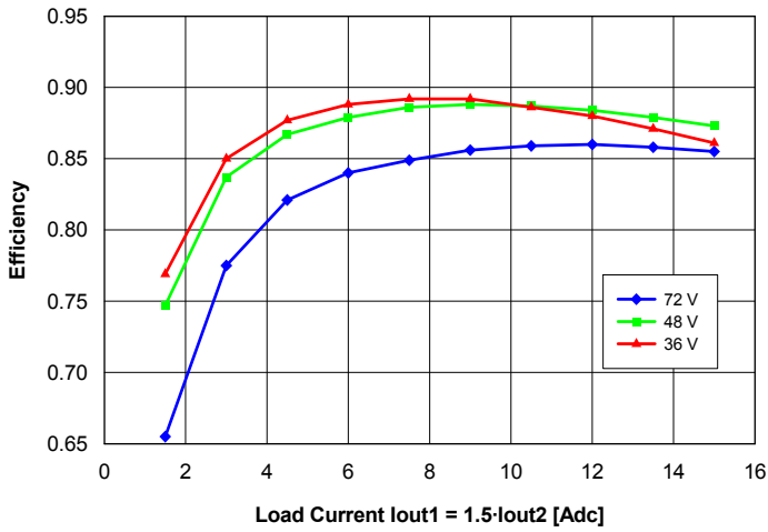
Fig. 20: Efficiency vs. balanced load current ( I_{out1} = 1.5 \cdot I_{out2} ) and input voltage for converter mounted vertically with air flowing from pin 3 to pin 1 at a rate of 300 LFM (1.5 m/s) and T_a = 25^\circ\text{C} .
