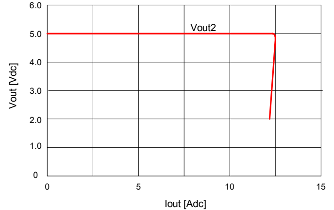
Fig. 31: Output voltage Vout2 vs. load current Iout2 showing current limit point and converter shutdown point. When Vout2 is in current limit, Vout1 will follow with less than 1 V difference until Vout2 reaches shut-down threshold of 2 V. Input voltage has almost no effect on Vout2 current limit characteristic.
