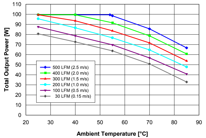
Fig. 13: Available output power for balanced load current (Iout1 = 1.5·Iout2) vs. ambient air temperature and airflow rates for converter mounted vertically with Vin = 48 V, air flowing from pin 4 to pin 3 and maximum FET temperature ≤ 120°C.
