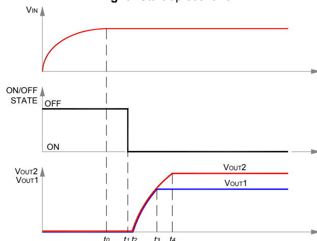
Fig. 6: Start-up scenario #2.
