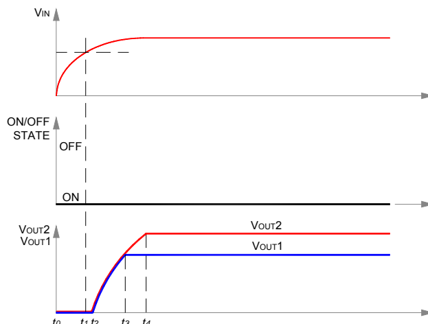
Fig. 5: Start-up scenario #1.
