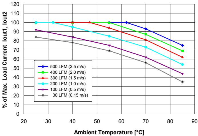
Fig. 10: Available balanced load current ( I_{out1} = 1.5 \cdot I_{out2} ) vs. ambient air temperature and airflow rates for converter mounted vertically with V_{in} = 48\text{ V} , air flowing from pin 3 to pin 1 and maximum FET temperature \leq 120^\circ\text{C} .
