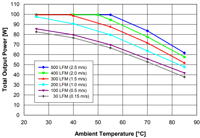
Fig. 12: Available output power for balanced load current (Iout1 = 1.5·Iout2) vs. ambient air temperature and airflow rates for converter mounted vertically with Vin = 48 V, air flowing from pin 3 to pin 4 and maximum FET temperature ≤ 120°C.
