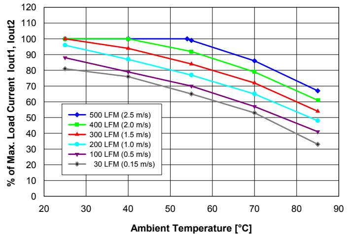
Fig. 15: Available balanced load current (Iout1 = 1.5·Iout2) vs. ambient air temperature and airflow rates for converter mounted vertically with Vin = 48 V, air flowing from pin 4 to pin 3 and maximum FET temperature ≤ 120°C.
