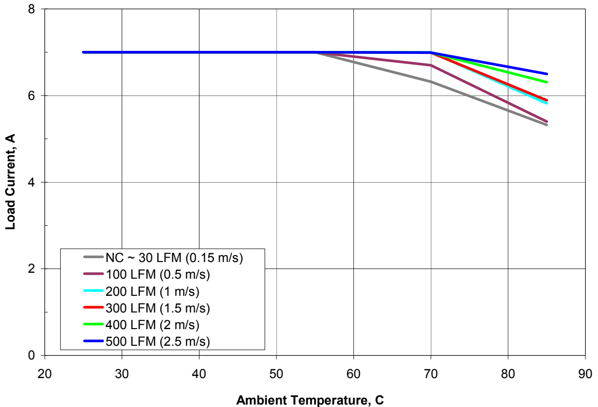
Figure 1. Available load current vs. ambient air temperature and airflow rates for SSQE48T07120 converter mounted vertically with air flowing from pin 1 to pin 3, Vin = 48 V. Note: NC – Natural convection
