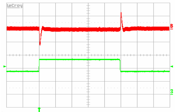
Figure 9. Output voltage response to load current step (3.5A–5.25A–3.5A) at V_{in}=48\text{V} . Top trace: output voltage (100 mV/div.). Bottom trace: load current (2A/div.). Current slew rate: 1A/ \mu\text{s} . C_o= 100\mu\text{F} Tantalum + 1 \mu\text{F} ceramic. Time scale: 0.2 ms/div.
