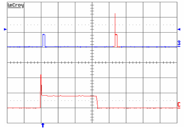
Figure 14. Load current (top trace, 5 A/div., 50 ms/div.) into a 10 \text{m}\Omega short circuit during restart, at V_{in} = 48 \text{ V} . Bottom trace (5 A/div., 2 ms/div.) is an expansion of the on-time portion of the top trace
