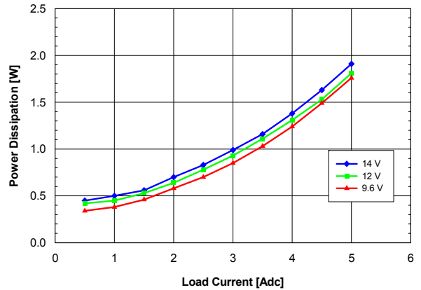
Fig. 2.0V.4: Power Loss vs. load current and input voltage for V_{out} = 2.0V converter mounted vertically with air flowing from pin 5 to pin 1 at a rate of 200 LFM (1 m/s) and T_a = 25^\circ C .
