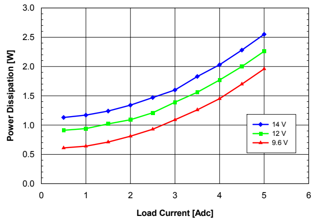
Fig. 5.0V.4: Power Loss vs. load current and input voltage for V_{out} = 5.0V converter mounted vertically with air flowing from pin 5 to pin 1 at a rate of 200 LFM (1 m/s) and T_a = 25\text{ }^{\circ}C .
