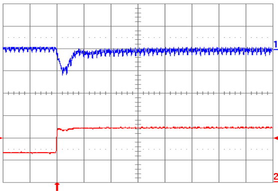
Fig. 1.0V.7: Output voltage response for V_{out} = 1.0V to a positive load current step change from 2.5A to 5A with a slew rate of 5A/\mu s at V_{in} = 12V . Top trace: output voltage (100mv/div); Bottom trace: load current (2A/div). C_o = 47\mu F ceramic. Time scale: 20 \mu s /div.
