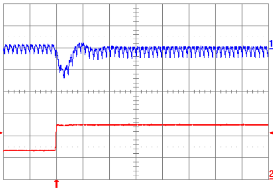
Fig. 3.3V.7: Output voltage response for V_{out} = 3.3V to a positive load current step change from 2.5A to 5A with a slew rate of 5A/\mu s at V_{in} = 12V . Top trace: output voltage (100mv/div); Bottom trace: load current (2A/div). C_o = 47\mu F ceramic. Time scale: 20 \mu s /div.
