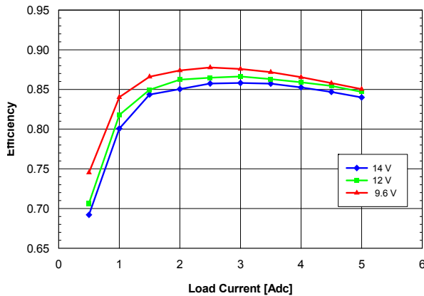
Fig. 2.0V.3: Efficiency vs. load current and input voltage for V_{out} = 2.0V converter mounted vertically with air flowing from pin 5 to pin 1 at a rate of 200 LFM (1 m/s) and T_a = 25^\circ C .
