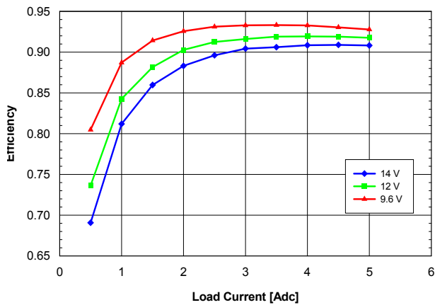
Fig. 5.0V.3: Efficiency vs. load current and input voltage for V_{out} = 5.0V converter mounted vertically with air flowing from pin 5 to pin 1 at a rate of 200 LFM (1 m/s) and T_a = 25\text{ }^{\circ}C .
