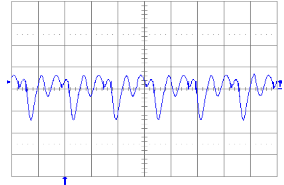
Fig. 1.8V.6: Output voltage ripple (10mv/div) at full rated load current into a resistive load with external capacitance 47\mu F ceramic + 1\mu F ceramic and V_{in} = 12V for V_{out} = 1.8V . Time scale: 2 \mu s /div.
