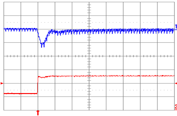
Fig. 1.2V.6: Output voltage response for V_{out} = 1.2V to a positive load current step change from 2.5A to 5A with a slew rate of 5A/\mu s at V_{in} = 12V . Top trace: output voltage (100mv/div); Bottom trace: load current (2A/div). C_o = 47\mu F ceramic. Time scale: 20 \mu s /div.
