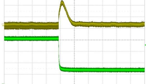
Figure 17 - Load transient V_1 , 45 to 20 A (500 \mu s/div) CH1: V_1 (200 mV/div) CH4: I_1 (10 A/div)
