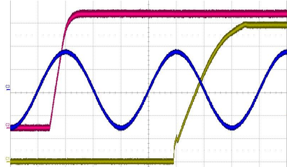
Figure 7 - Turn-On AC Line 230VAC, full load (5ms/div) CH1: V_1 (2V/div) CH2: V_{SB} (1V/div) CH3: V_{in} (200V/div)
