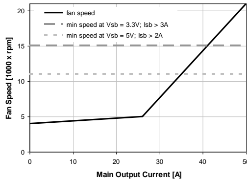
Figure 38 - Fan speed vs. main output load
