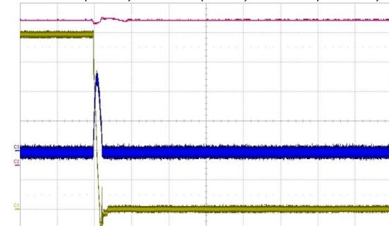
Figure 9 - Short circuit on V_1 (500 \mu s/div) CH1: V_1 (2 V/div) CH2: V_{SB} (1 V/div) CH3: I_1 (200 A/div)
