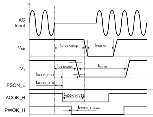
Figure 27 - AC long dips
