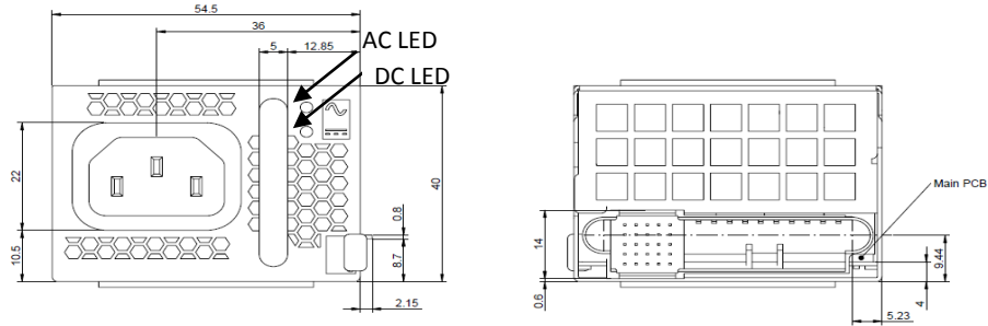
Figure 44 - Front and Rear View
