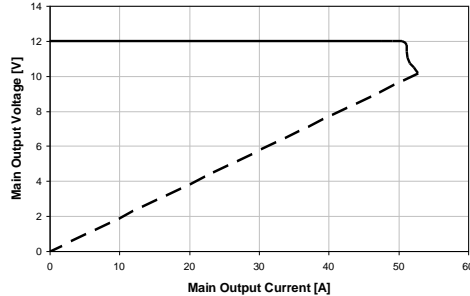
Figure 18 - Current Limitation on V_1 ( V_i = 230 VAC)
