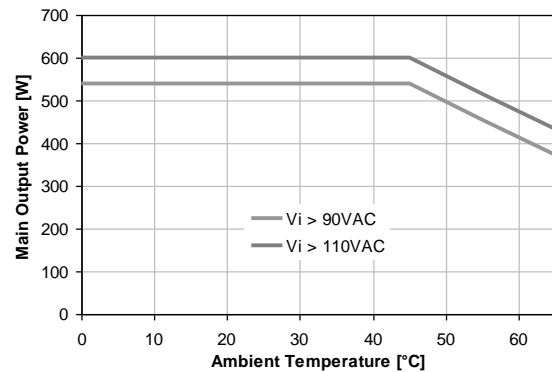
Figure 40 - Thermal derating for PFE600-12-054RA
