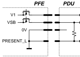
Figure 24 - PRESENT_L signal pin
