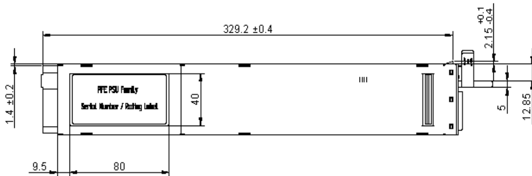
Figure 42 - Top View
