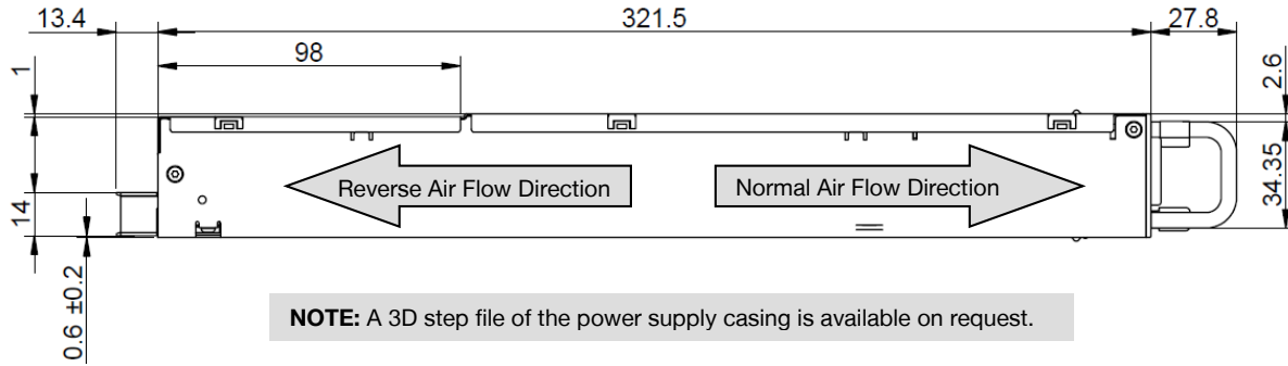
Figure 41 - Side View 1
