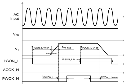
Figure 28 - PSON_L turn-on/off timing
