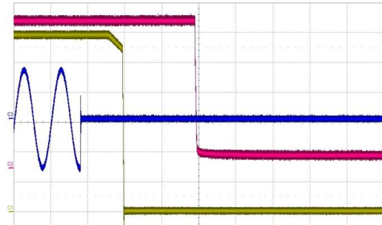
Figure 8 - Turn-Off AC Line 230 VAC, full load (20 ms/div) CH1: V_1 (2 V/div) CH2: V_{SB} (1 V/div) CH3: V_{in} (200 V/div)
