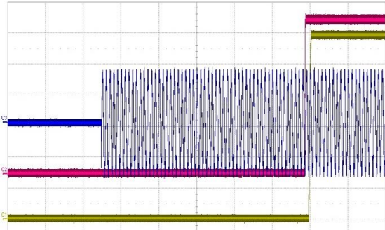
Figure 6 - Turn-On AC Line 230VAC, full load (200ms/div) CH1: V_1 (2V/div) CH2: V_{SB} (1V/div) CH3: V_{in} (200V/div)
