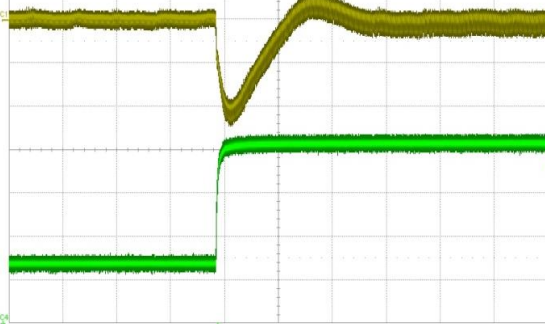
Figure 16 - Load transient V_1 , 20 to 45 A (500 \mu s/div) CH1: V_1 (200 mV/div) CH4: I_1 (10 A/div)
