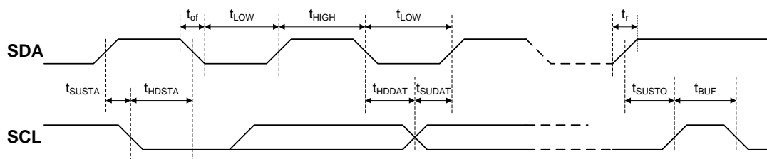
Figure 33 - I 2 C / SMBus Timing
