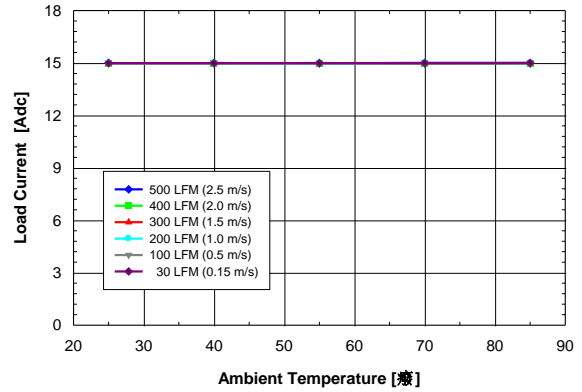
Figure 4. Available output current vs. ambient air temperature and airflow rates for converter DP7120G mounted horizontally with air flowing from input to output, MOSFET temperature \leq 120^\circ\text{C} , V_{in} = 12\text{ V} , V_{out} = 5\text{ V} , and F_{sw} = 1\text{MHz}
