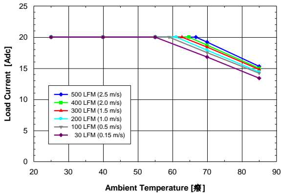
Figure 3. Available output current vs. ambient air temperature and airflow rates for converter DP7120G mounted horizontally with air flowing from input to output, MOSFET temperature \leq 120^\circ\text{C} , V_{in} = 12\text{ V} , V_{out} = 5\text{ V} , and F_{sw} = 500\text{KHz}
