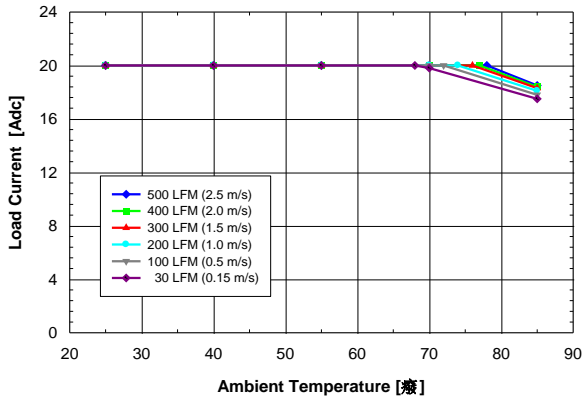
Figure 3. Available output current vs. ambient air temperature and airflow rates for converter DP7120G mounted horizontally with air flowing from input to output, MOSFET temperature \leq 120^\circ\text{C} , V_{in} = 12\text{ V} , V_{out} = 5\text{ V} , and F_{sw} = 500\text{KHz}
