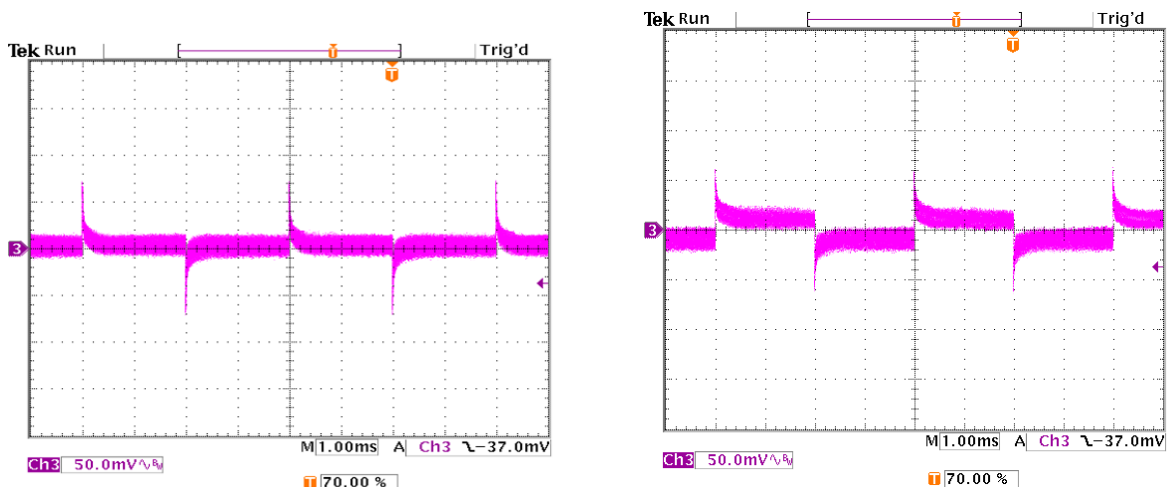
Figure 52. Transient Response with Regulation set to 0.0 mV/A. Figure 53. Transient Response with Regulation set to 0.74 mV/A
