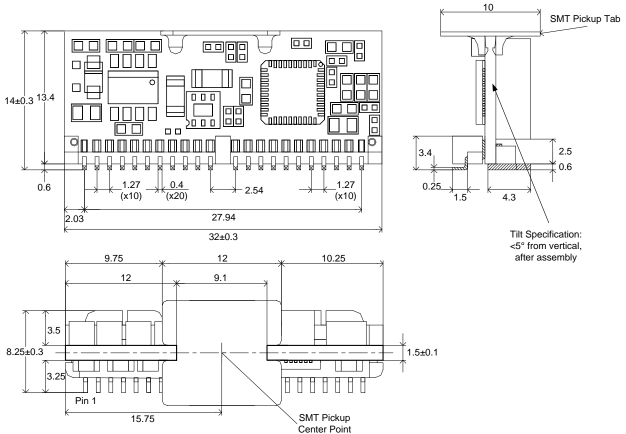
Figure 60. Mechanical Drawing
