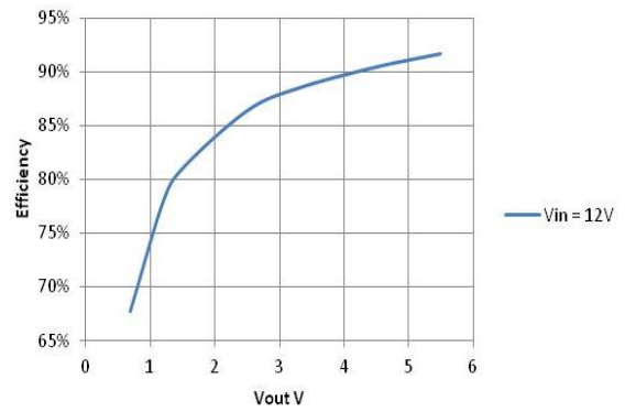
Figure 8. Efficiency vs. Output Voltage, Iout=7A, Fsw=500kHz
