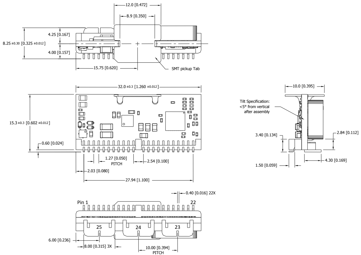
Figure 55: Mechanical Drawing
