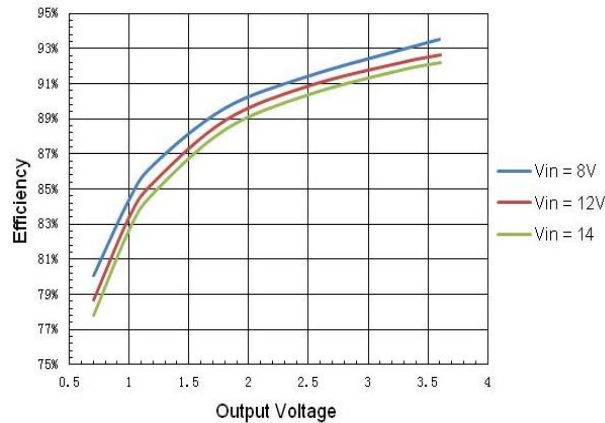
Figure 7: Efficiency vs. Output voltage for converter DP7130, with 30A load, input voltage at 8, 12 and 14V, at T_a = 25\text{ }^\circ\text{C} .
