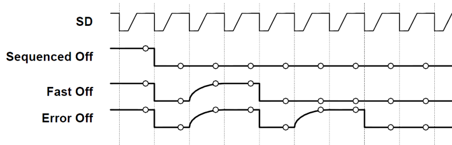
Figure 39. OK Severity Encoding Waveforms
