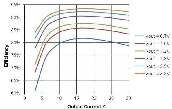
Figure 6: Efficiency vs. load current and input voltage for converter DP7130G at 12\text{ V in} , T_a = 25^\circ\text{C} .
