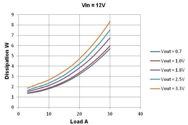
Figure 9: Power dissipation vs. load for converter DP7130, with V_{in} = 12V in T_a = 25\text{ }^\circ\text{C} .
