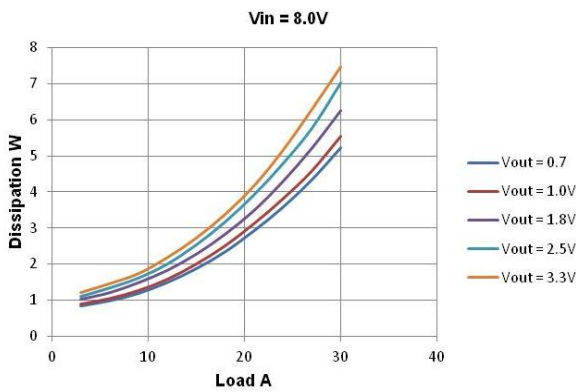
Figure 8: Power dissipation vs. load for converter DP7130, with V_{in} = 8.0V in T_a = 25\text{ }^\circ\text{C} .
