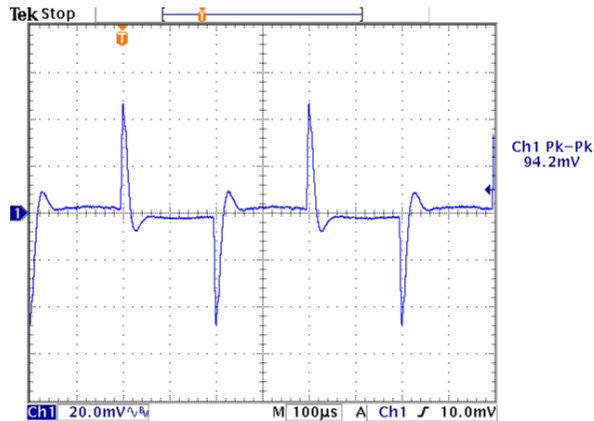
Figure 13. Transient Response with Regulation set to 0 mV/A.
