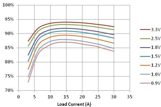
Figure 5: Efficiency vs. load current and output voltage for converter DP7130G at 8\text{ V in} , T_a = 25^\circ\text{C} .
