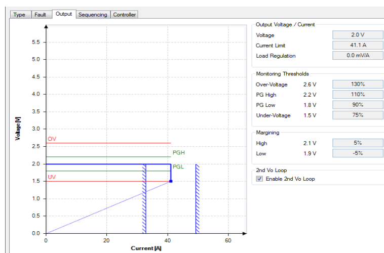
Figure 10. Output Configuration Window
