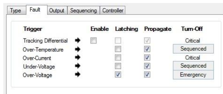
Figure 30. dPOL Fault Propagation Option Window
