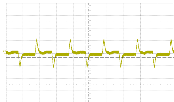
Fig. 11: Output voltage response to load current step-change (10 A – 15 A – 10 A) at V_{in} = 48\text{ V} . Current slew rate: 0.1 A/ \mu\text{s} . C_o = 470\mu\text{F} E-cap + 1 \mu\text{F} ceramic + 10 \mu\text{F} tantalum. Time scale: 500 \mu\text{s} /div.
