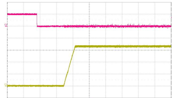
Fig. 10: Turn-on transient at full rated load current (resistive) plus 4700 \mu\text{F} at V_{in} = 48\text{ V} , triggered via ON/OFF pin. Top trace: ON/OFF signal (5 V/div.). Bottom trace: output voltage (1 V/div.). Time scale: 50 ms/div.
