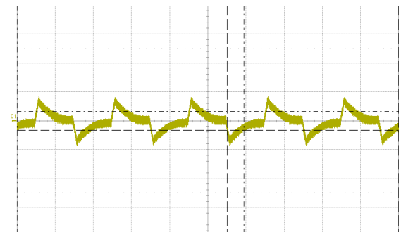
Fig. 12: Output voltage response to load current step-change (10 A – 15 A – 10 A) at V_{in} = 48\text{ V} . Current slew rate: 0.1 A/ \mu\text{s} . C_o = 4700\mu\text{F} E-cap + 1 \mu\text{F} ceramic + 10 \mu\text{F} tantalum. Time scale: 500 \mu\text{s} /div.
