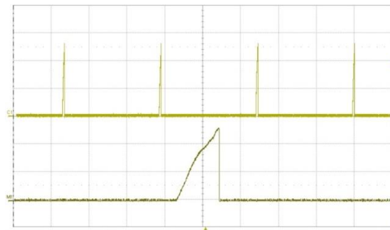
Fig. 17: Load current (top trace, 20 A/div., 200 ms/div.) into a 10 \text{ m}\Omega short circuit during restart, at V_{in} = 48 \text{ V} . Bottom trace (20 A/div., 10 ms/div.) is an expansion of the on-time portion of the top trace.
