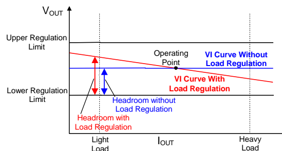
Figure 8. Optimal Voltage Positioning Concept
