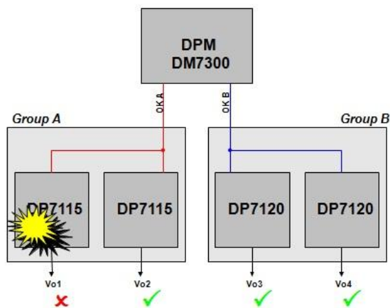
Figure 31. No Group Fault Propagation
