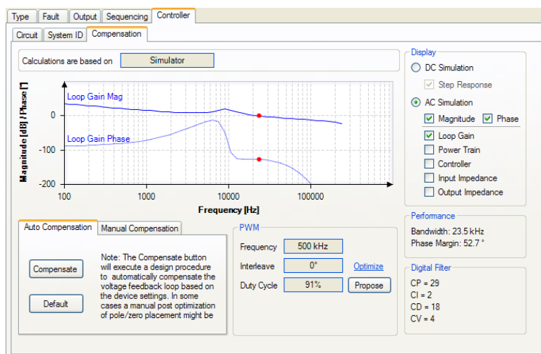
Figure 36. PWM Controller Window
