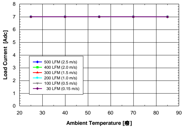
Figure 1. Available output current vs. ambient air temperature and airflow rates for converter DP7010G mounted horizontally with air flowing from input to output, MOSFET temperature \leq 120\text{ }^{\circ}\text{C} , V_{in} = 12\text{ V} , V_{out} = 5\text{ V} , and F_{sw} = 500\text{ KHz}
