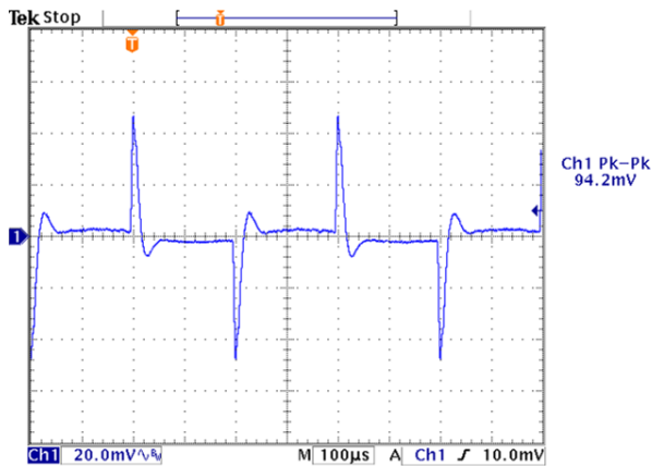
Figure 9 Transient Response with Regulation set to 0 mV/A.
