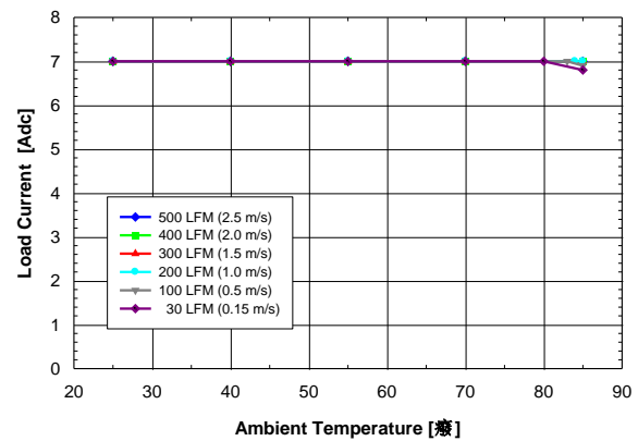
Figure 2 Available output current vs. ambient air temperature and airflow rates for converter DP7010G mounted horizontally with air flowing from input to output, MOSFET temperature \leq 120\text{ }^{\circ}\text{C} , V_{in} = 12\text{ V} , V_{out} = 5\text{ V} , and F_{sw} = 1\text{ MHz}
