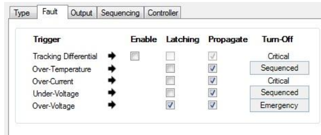
Figure 26 GUI dPOL Fault Propagation Option Window
