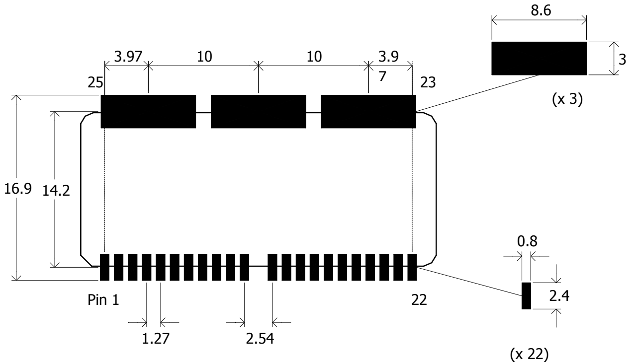
Figure 52. Recommended PCB Pad Sizes
