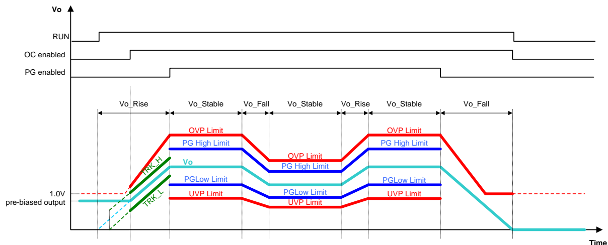
Figure 25. Protection Enable Conditions
