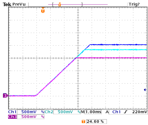
Figure 16. Tracking Turn-On. Rising Slew Rate is Programmed at 0.5V/ms for each output.
