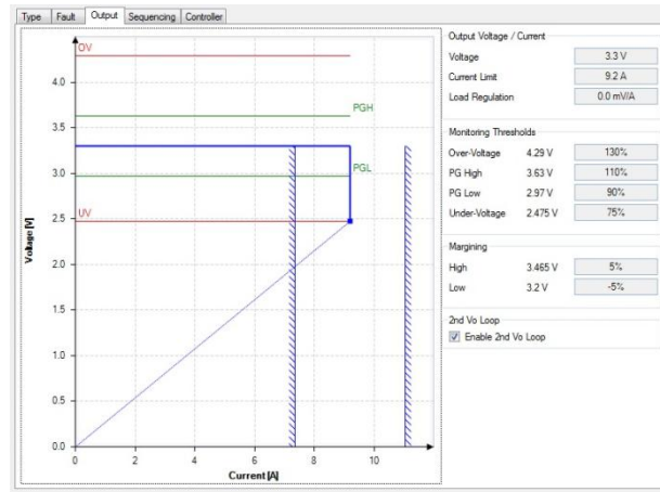
Figure 6. Output Configuration Window
