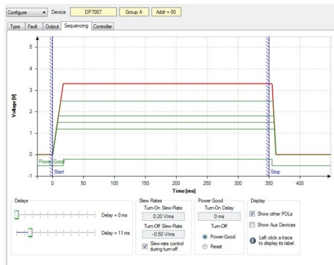
Figure 11. dPOL Configure Sequencing Window
