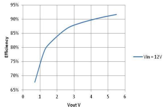
Figure 4 Efficiency vs. Output Voltage, I_{out} = 7\text{ A} , F_{sw} = 500\text{ kHz}
