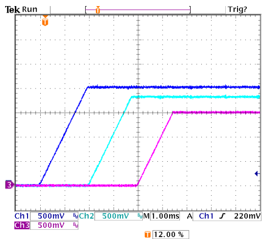
Figure 18. Sequenced Turn-On. Rising Slew Rate is Programmed at 1V/ms. V2 Delay is 2ms, V3 delay is 4ms.
