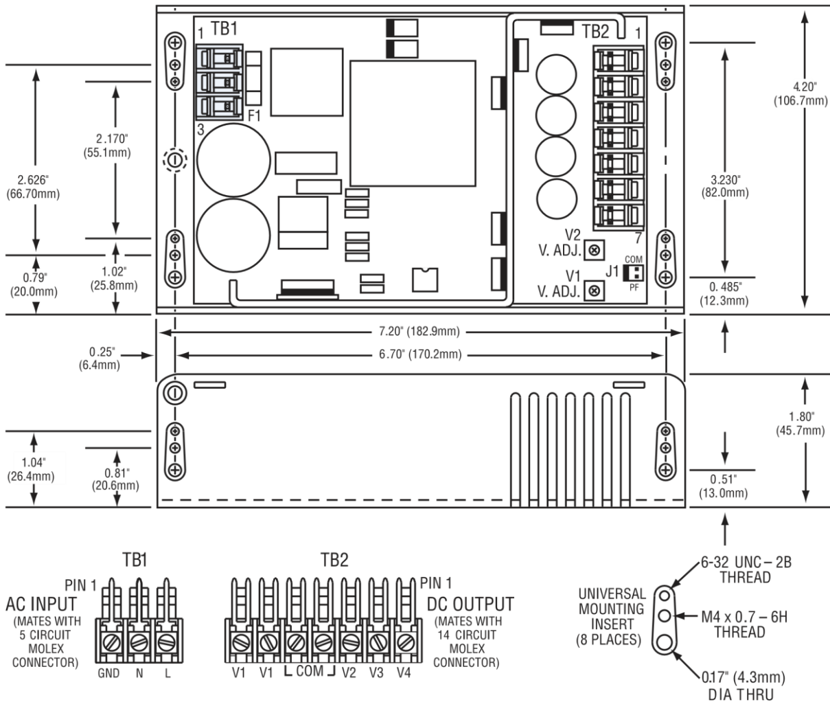
Figure-1 - Mechanical Drawing
