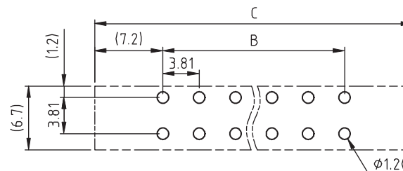
RECOMMENDED PCB LAYOUT - COMPONENT VIEW
