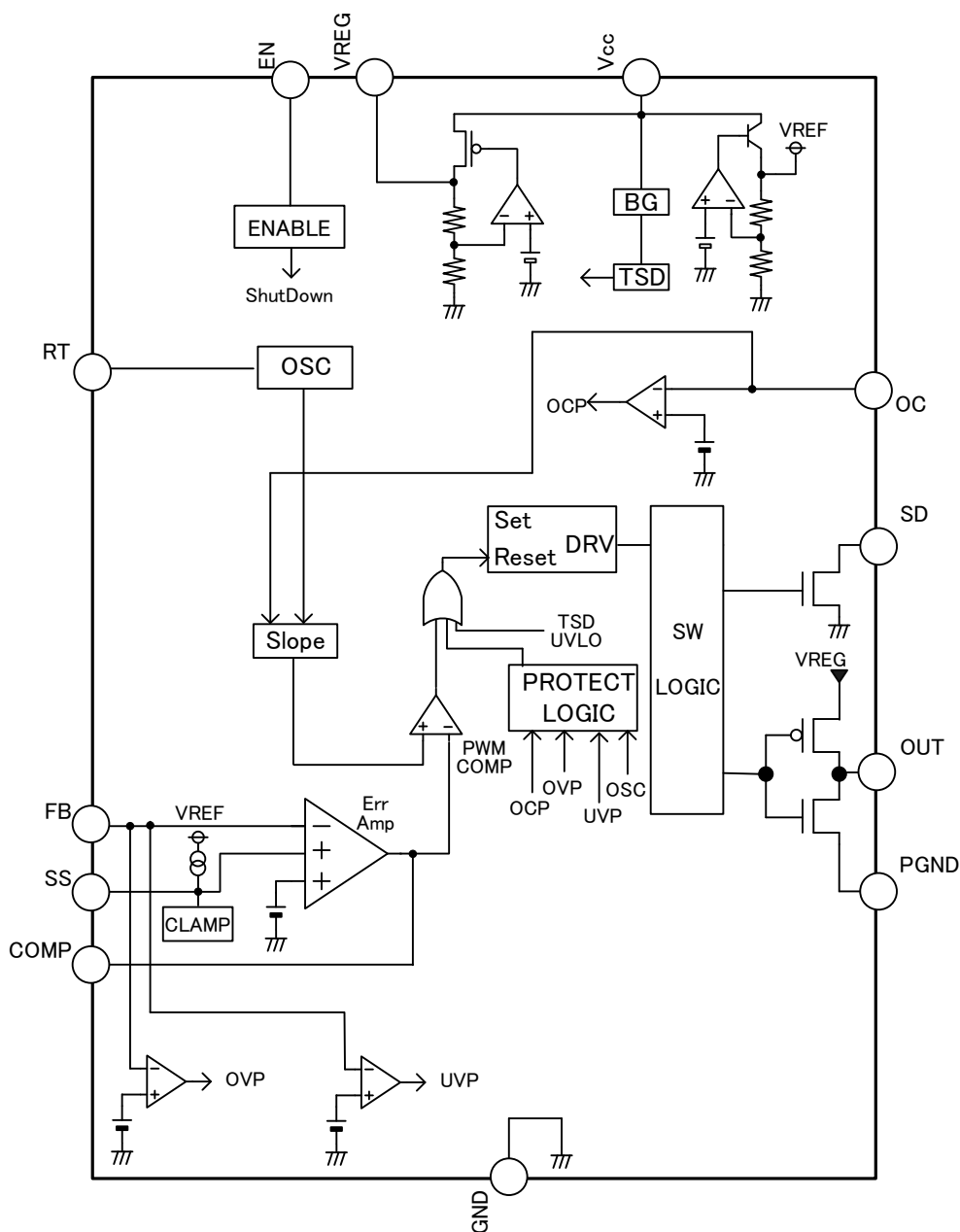
Figure 3. Block Diagram
