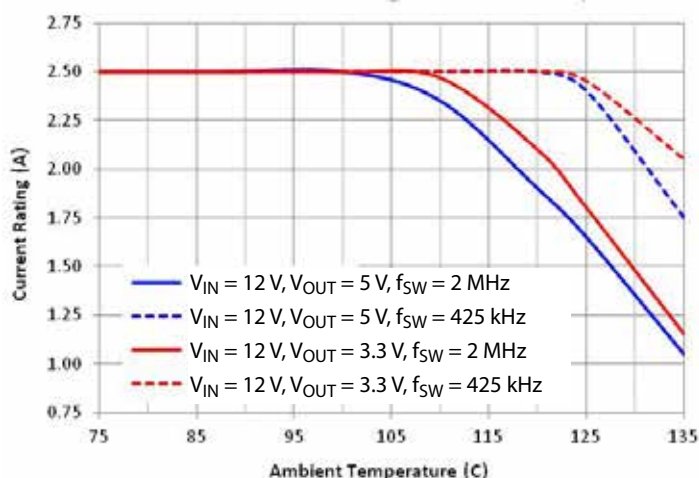
Figure 1: A8580 Typical Current Derating
