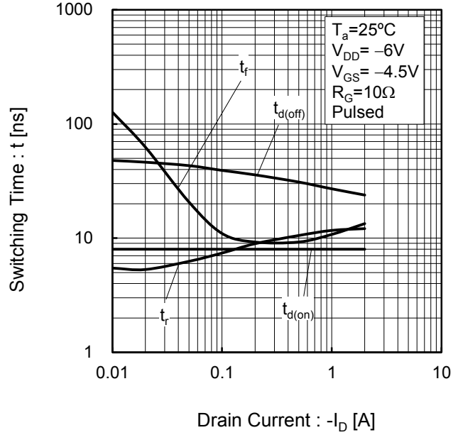
Fig.20 Switching Characteristics
