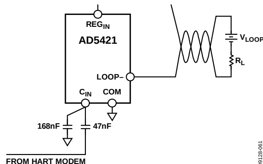
Figure 49. Circuit Diagram for Figure 48
