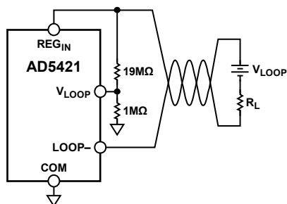
Figure 42. Resistor Divider Connection at V_{\text{LOOP}} Pin
