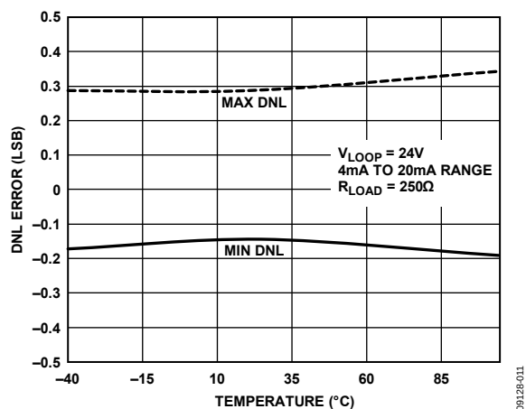
Figure 13. Differential Nonlinearity Error vs. Temperature
