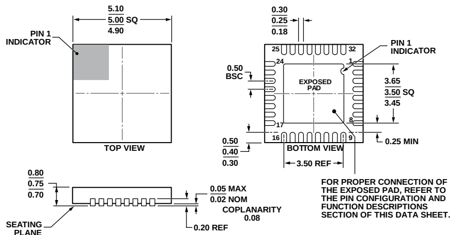
Figure 54. 32-Lead Lead Frame Chip Scale Package [LFCSP_WQ] 5 mm × 5 mm Body, Very Very Thin Quad (CP-32-11) Dimensions shown in millimeters
