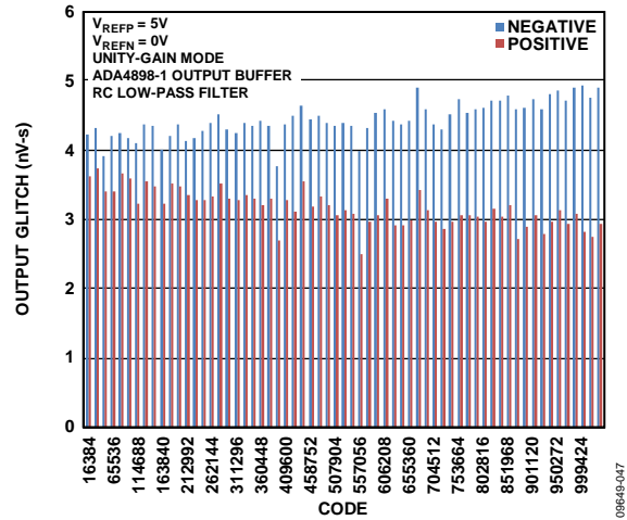
Figure 44. 6 MSB Segment Glitch Energy for 5 V V_{REF}
