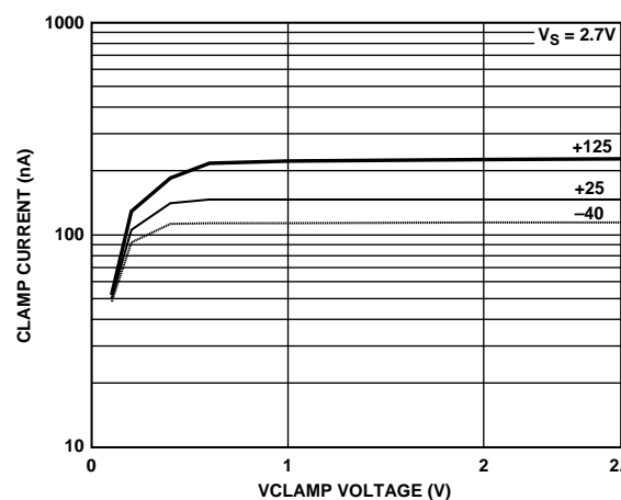
Figure 15. VCLAMP Current Over Temperature at V_S = 2.7\text{V} vs. VCLAMP Voltage
