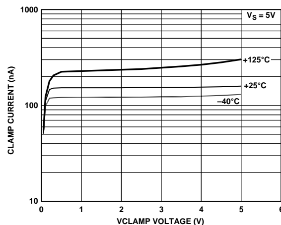
Figure 14. VCLAMP Current Over Temperature at V_S = 5\text{V} vs. VCLAMP Voltage
