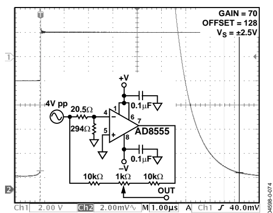
Figure 47. Settling Time 0.01%
