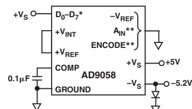
Burn-In Connections
