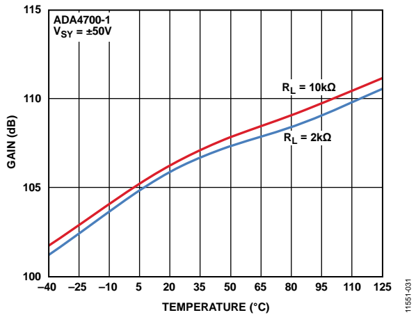
Figure 26. Open-Loop Gain vs. Temperature for Various Load Resistances, V SY = ±50 V
