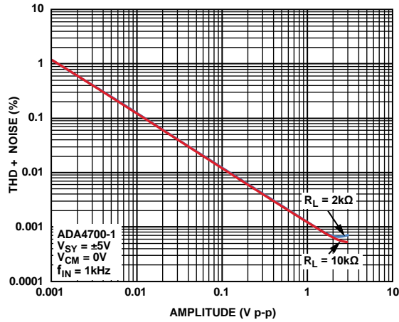
Figure 31. Total Harmonic Distortion + Noise (THD + Noise) vs. Amplitude, V SY = ±5 V
