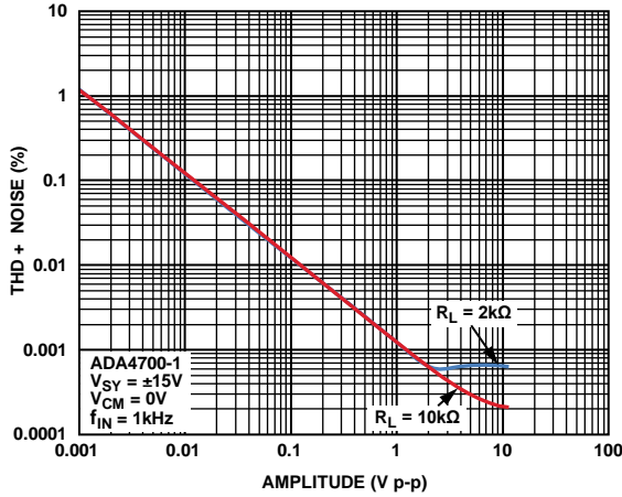
Figure 32. Total Harmonic Distortion + Noise (THD + Noise) vs. Amplitude, V SY = ±15 V
