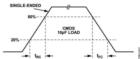
Figure 2. CMOS Timing, Single-Ended, 10 pF Load
