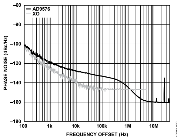
Figure 8. Phase Noise (OUT2)— f_{OUT2} = 156.25 MHz (HSTL)
