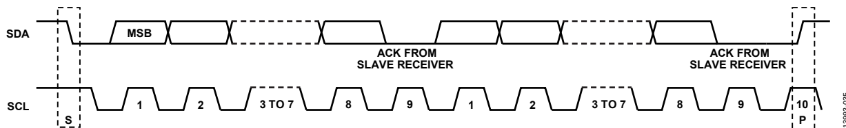
Figure 35. Acknowledge Bit
