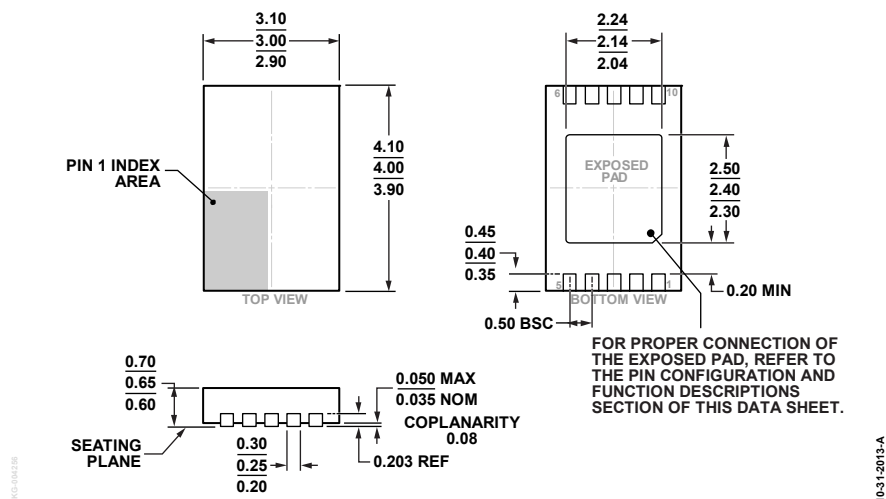
Figure 18. 10-Lead Lead Frame Chip Scale Package [LFCSP] 3 mm × 4 mm Body and 0.65 mm Package Height (CP-10-33) Dimensions shown in millimeters
