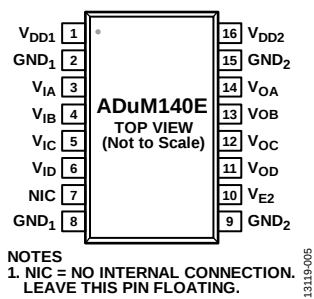
Figure 7. ADuM140E Pin Configuration
