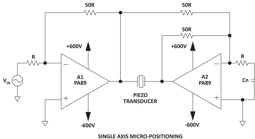
Figure 16: Typical Application
