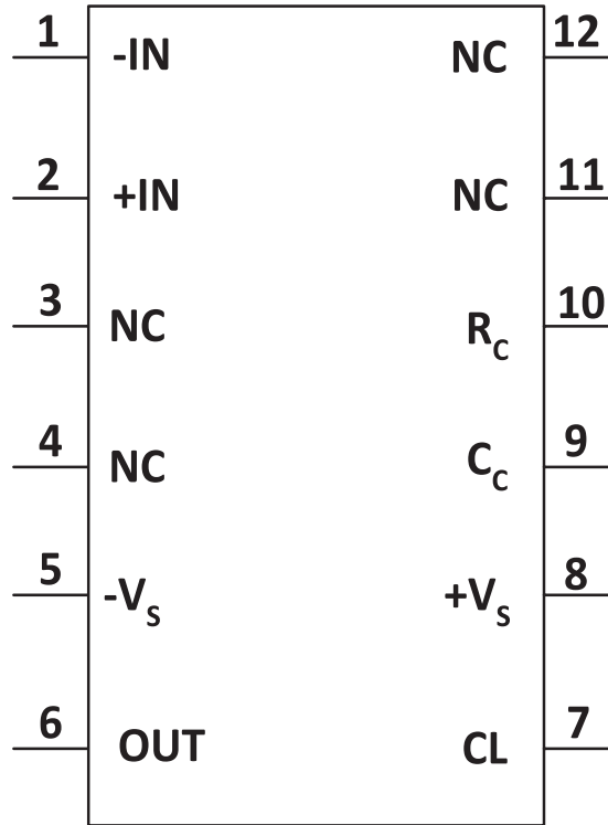
Figure 2: External Connections
