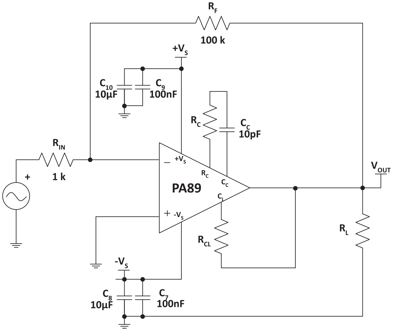
Figure 1: Typical Connection
