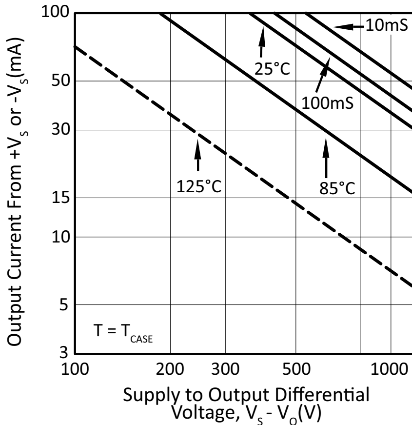
Figure 15: SOA
