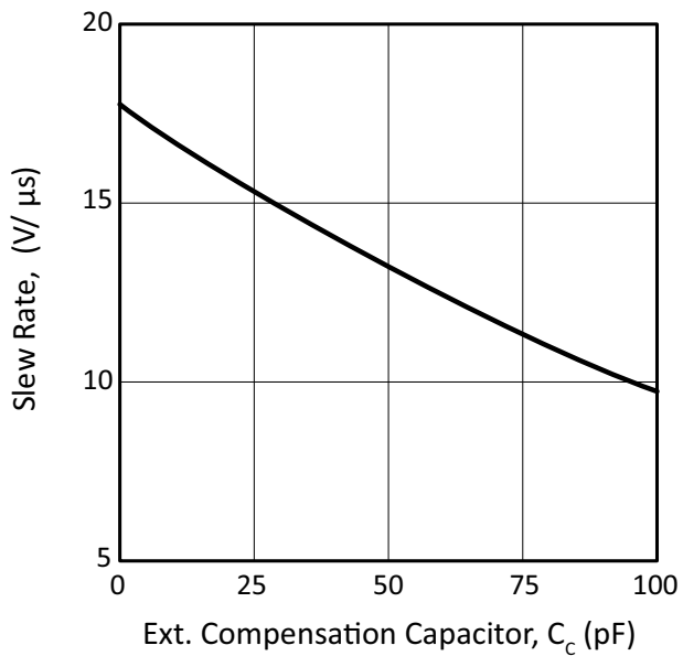
Figure 9: Slew Rate vs. Comp
