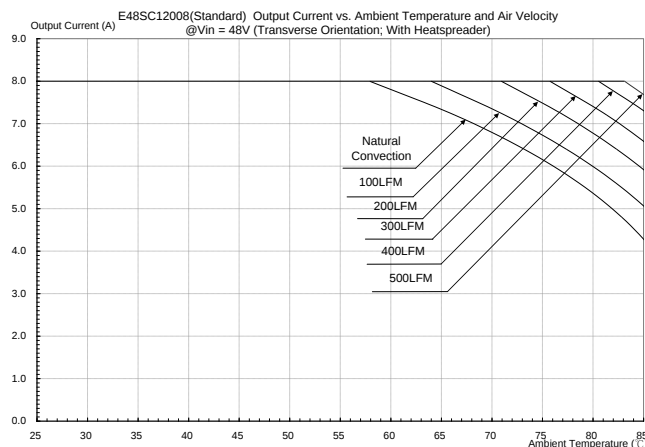
Figure 22: Output current vs. ambient temperature and air velocity @Vin=48V (Transverse Orientation, airflow from Vin+ to Vin-,with heat spreader)
