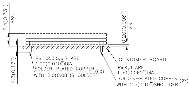
SIDE VIEW
