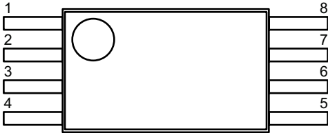
Package LE, 8-Pin TSSOP Pin-out Diagram
