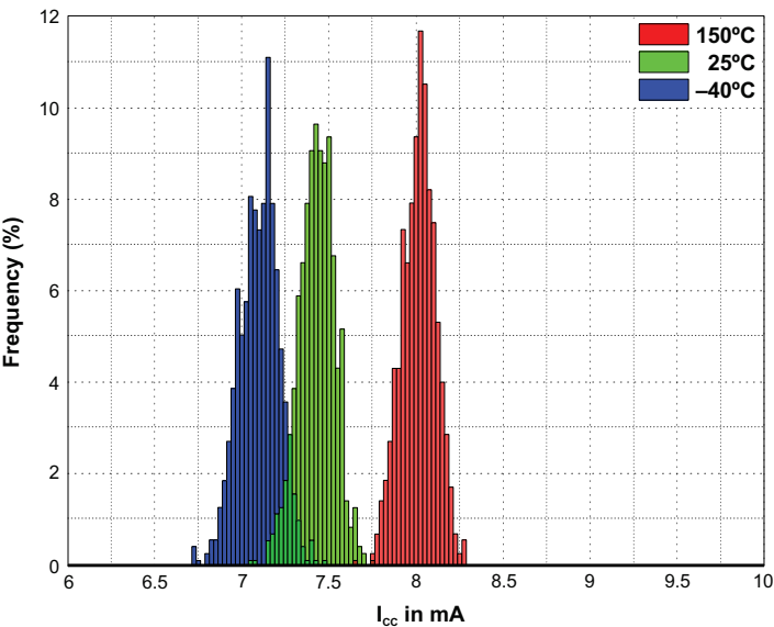
Figure 14: I_{CC} Distribution Over Temperature ( V_{CC} = 14.5\text{ V} )
