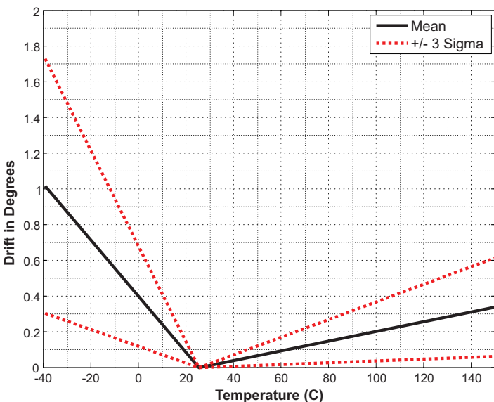
Figure 9: Temperature Drift (300 G)
