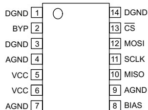
LE-14 Package (Single SoC)
