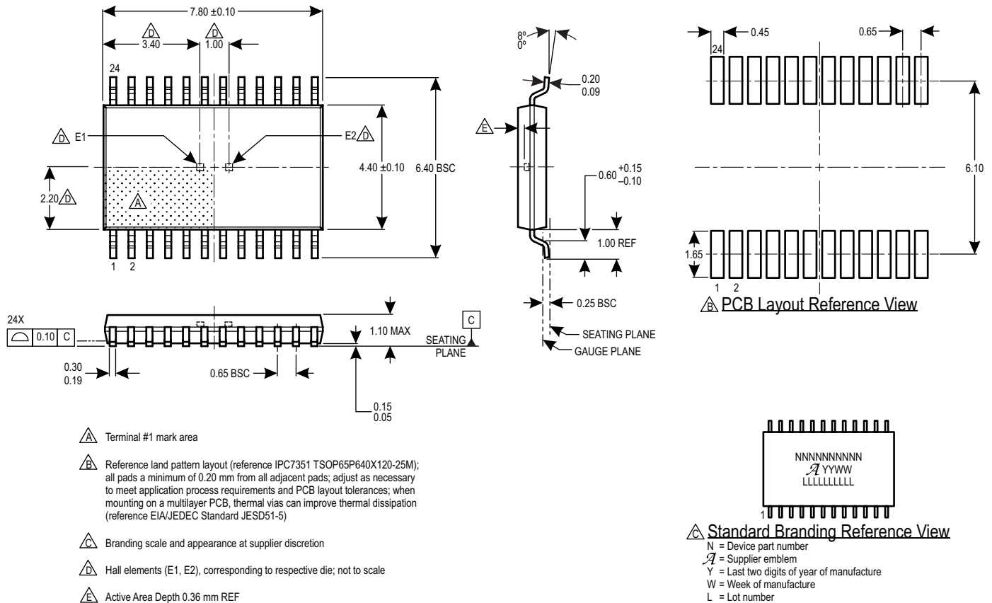
Figure 19: Package LE, 24-Pin TSSOP (Dual Die Version)
