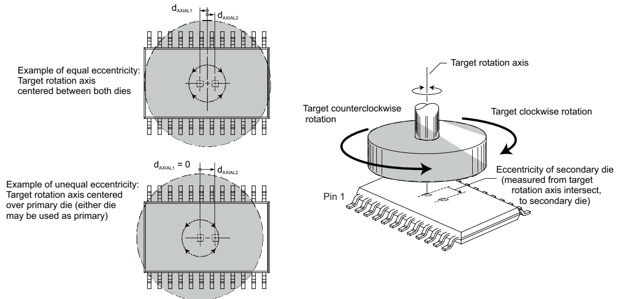
Figure 5: Demonstration of Magnet to Sensing Element Eccentricity (dual die version used as example)
