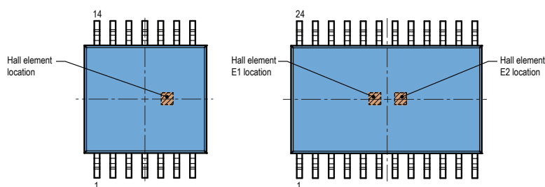
Figure 17: Hall Element Located Off-Center within the Device Body Refer to the Package Outline Drawing for reference dimensions.
