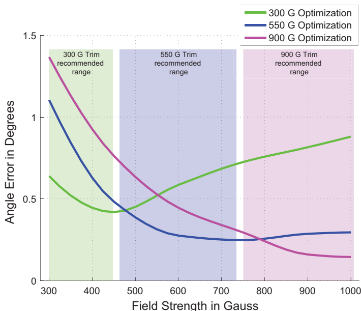
Figure 3: Maximum Peak Angle Error Over Field Strength Different Factory Optimizations
