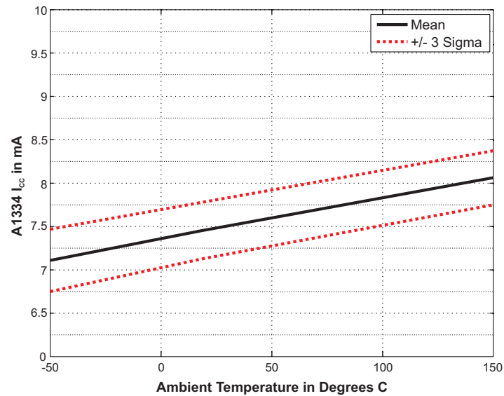
Figure 15: I_{CC} Over Temperature ( V_{CC} = 14.5\text{ V} )
