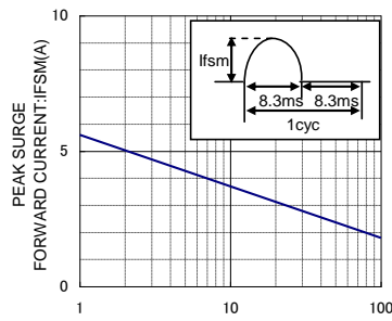
IFSM-CYCLE CHARACTERISTICS
