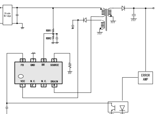
Figure 16(b). DC voltage monitor setting
