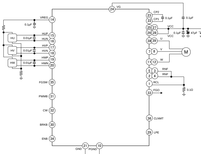
Figure 1. Application Circuit
