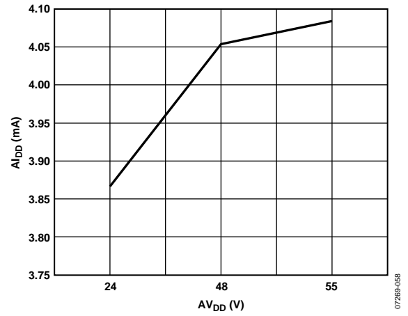
Figure 49. A_{I_{DD}} vs. AV_{DD} , I_{OUT} = 0 mA
