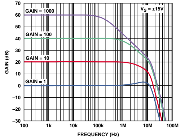
Figure 20. Gain vs. Frequency
