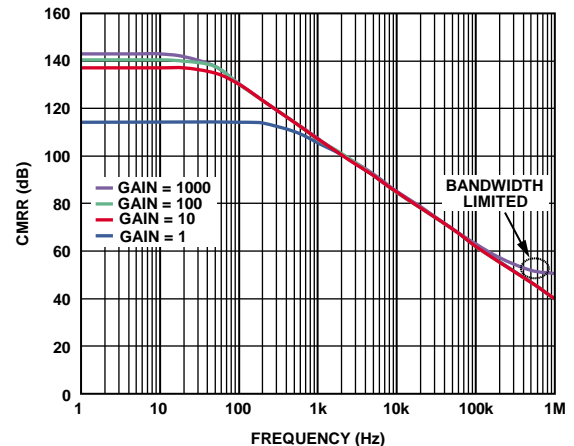
Figure 22. CMRR vs. Frequency, 1 kΩ Source Imbalance
