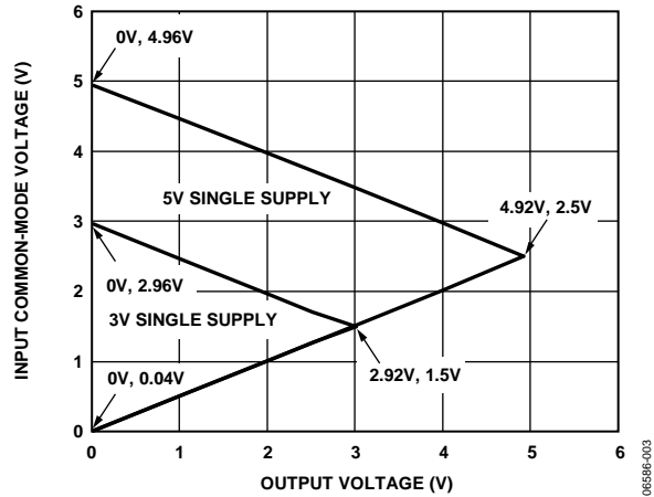
Figure 12. Instrumentation Amplifier Input Common-Mode Range vs. Output Voltage, All Gains, V_{REF} = 0\text{ V}
