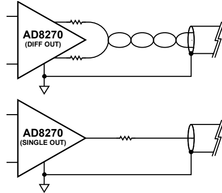
Figure 50. Driving Cabling
