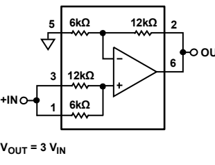
Figure 47. Noninverting Amplifier, G = 3
