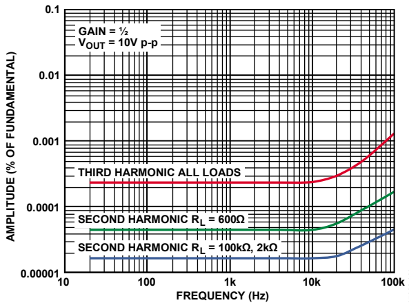
Figure 36. Harmonic Distortion Products vs. Frequency, G = \frac{1}{2}
