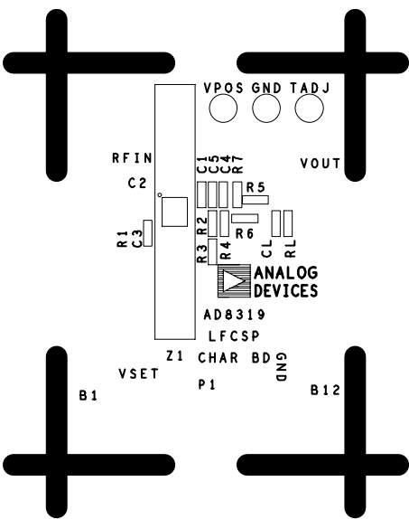
Figure 38. Component Side Silkscreen
