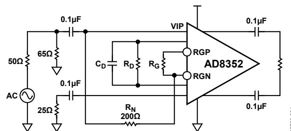
Figure 26. Single-Ended Schematic
