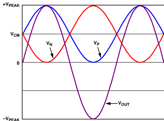
Figure 68. Output Voltage Waveforms
