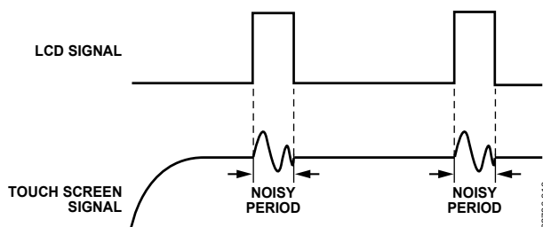
Figure 32. Effect of LCD Noise on Touch Screen Measurements
