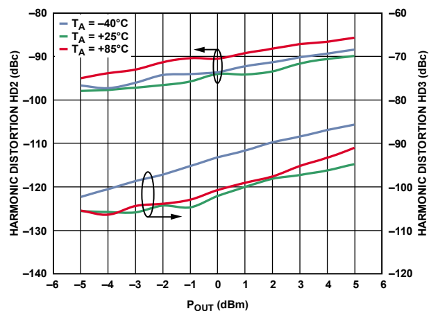
Figure 22. Harmonic Distortion vs. Power, Frequency = 140 MHz, Three Temperatures
