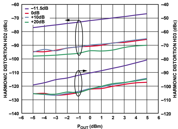
Figure 21. Harmonic Distortion vs. Power at Four Gain Codes, Frequency = 140 MHz
