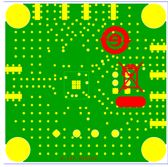
Figure 53. Evaluation Board Bottom Layer
