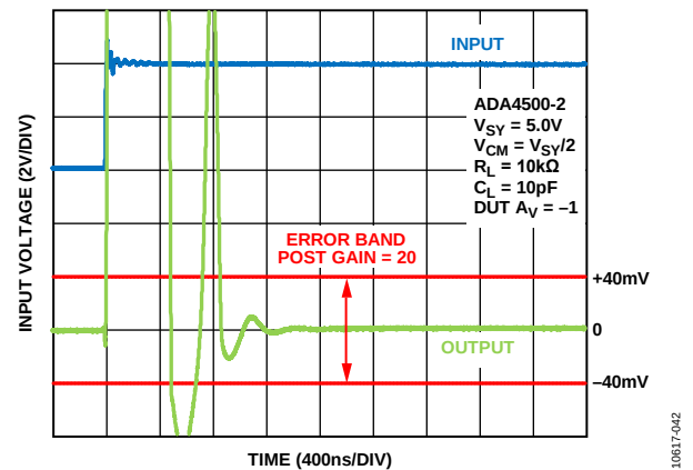
Figure 47. Positive Settling Time to 0.1%, V SY = 5.0 V
