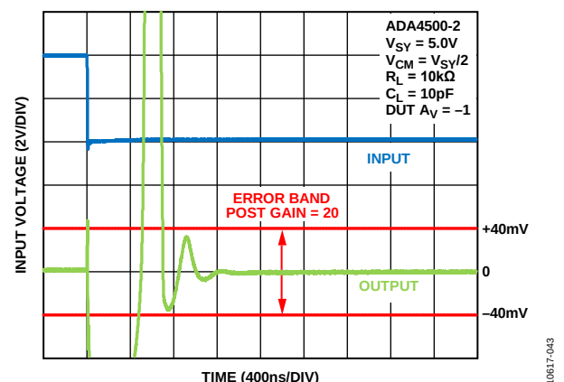
Figure 48. Negative Settling Time to 0.1%, V SY = 5.0 V
