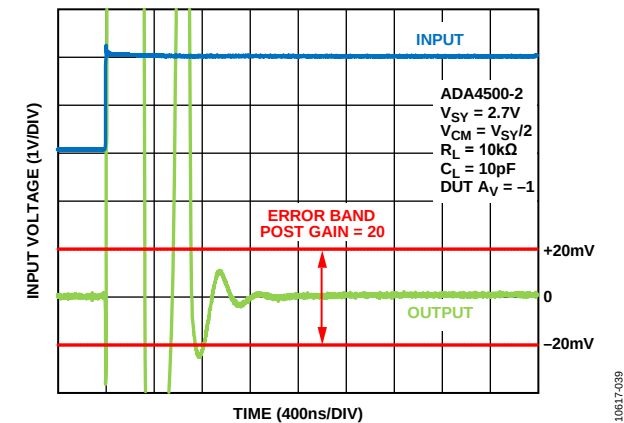
Figure 45. Positive Settling Time to 0.1%, V SY = 2.7 V
