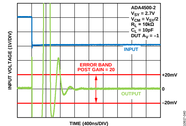
Figure 46. Negative Settling Time to 0.1%, V SY = 2.7 V
