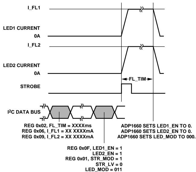
Figure 19. Flash Operation: Edge-Sensitive Mode
