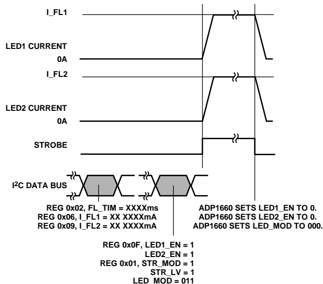
Figure 18. Flash Operation: Level-Sensitive Mode
