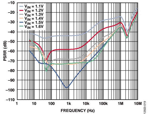
Figure 19. Power Supply Rejection Ratio (PSRR) vs. Frequency for Various Loads, V_{OUT} = 0.9\text{ V} , Load Current = 3 A
