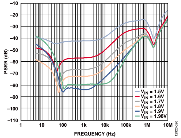
Figure 20. Power Supply Rejection Ratio (PSRR) vs. Frequency for Various Loads, V_{OUT} = 1.3\text{ V} , Load Current = 3 A
