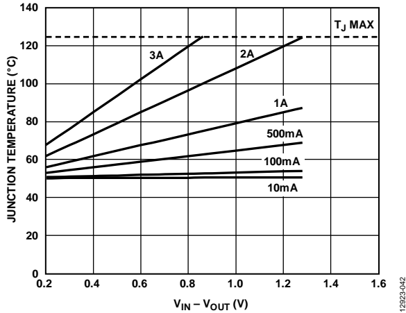
Figure 44. 1000 mm 2 of PCB Copper, T_B = 50^\circ\text{C} , LFCSP
