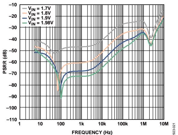
Figure 21. Power Supply Rejection Ratio (PSRR) vs. Frequency for Various Loads, V_{OUT} = 1.5\text{ V} , Load Current = 3 A
