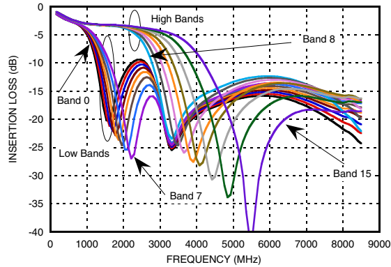
Figure 45. Insertion loss of the low pass filter.
