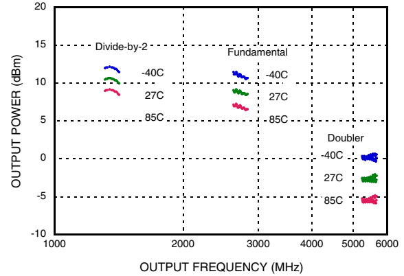
Typical Output Power - Narrow Band Match
