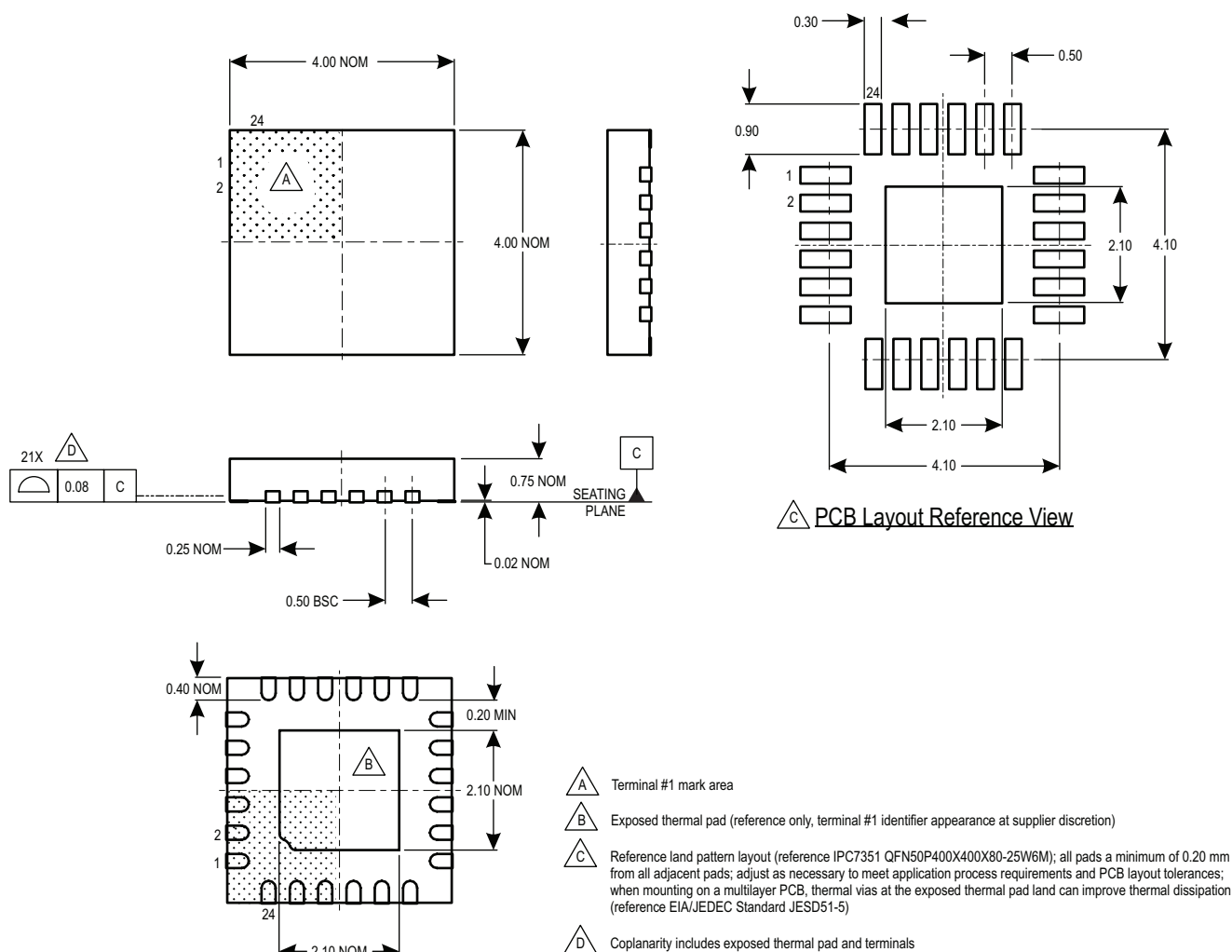
Figure 20: Package ES, 24-Pin 4 mm × 4 mm QFN with Exposed Thermal Package
