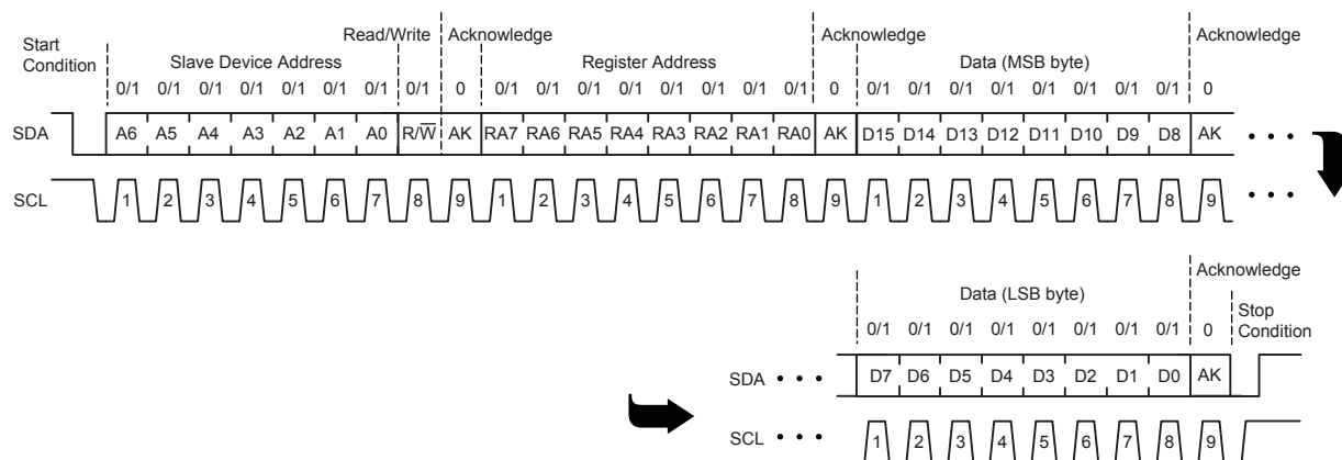
Figure A-2. Complete data transfer pulse train
