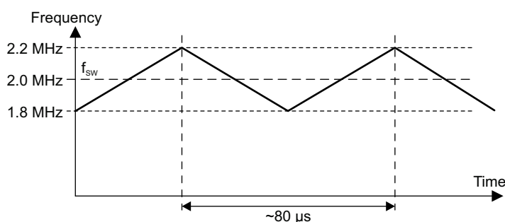
Figure 11: Switching Frequency Varied Linearly
