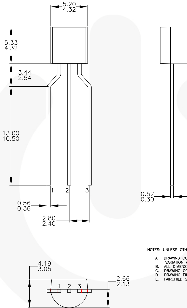
Figure 6. 3-LEAD, TO-92, MOLDED 0.200 IN-LINE SPACING LD FORM
