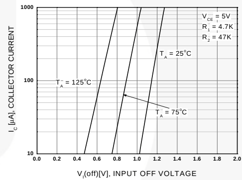
Figure 4. Input-Off Voltage
